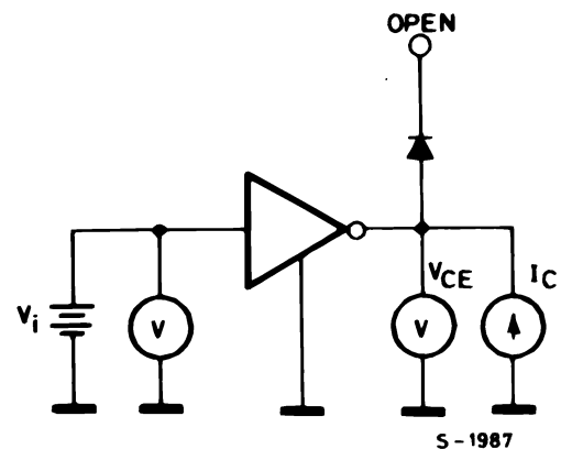
Figure 8. Input voltage
