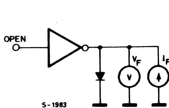
Figure 10. Clamp diode forward voltage
